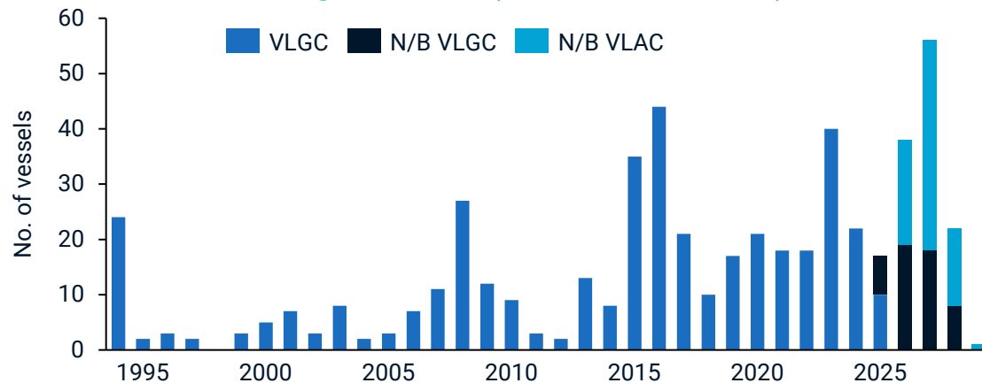
VLGC/VLAC Fleet Age Profile (Number of units)
